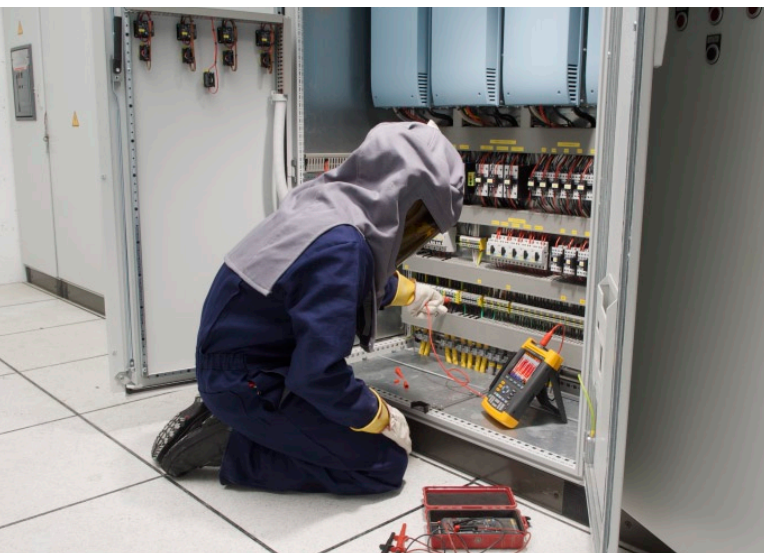
Rob Withey uses a Fluke ScopeMeter to check the output voltage that drives Peak 2 Peak conveyor motors.
